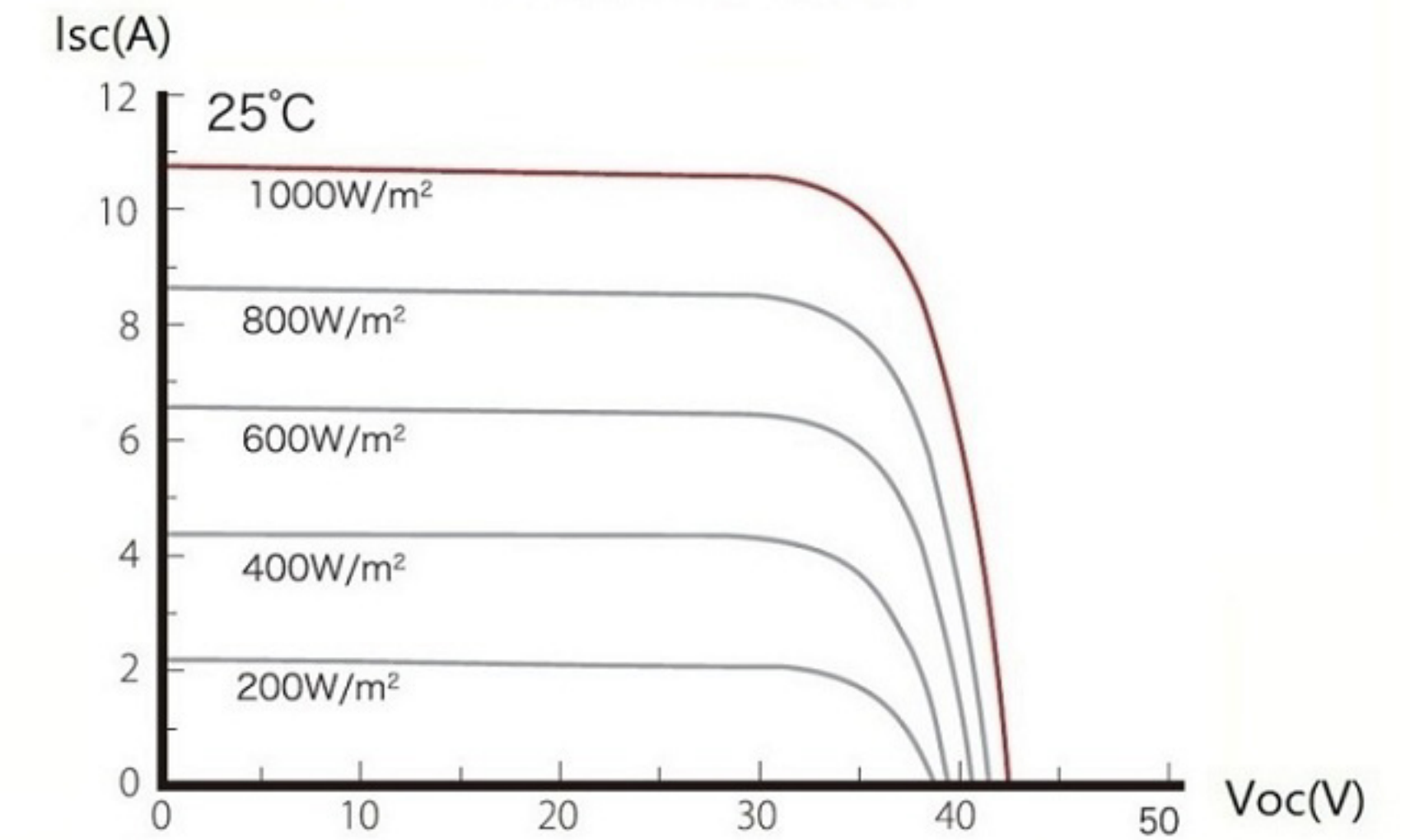
I-V Curves of PV module MS 360M-120 at various solar irradiance
