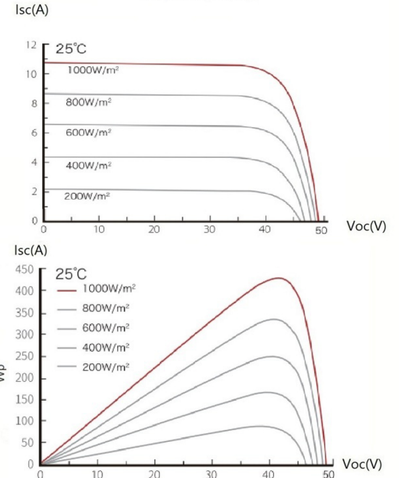
I-V Curves of PV module MS 430M-144 at various solar irradiance
